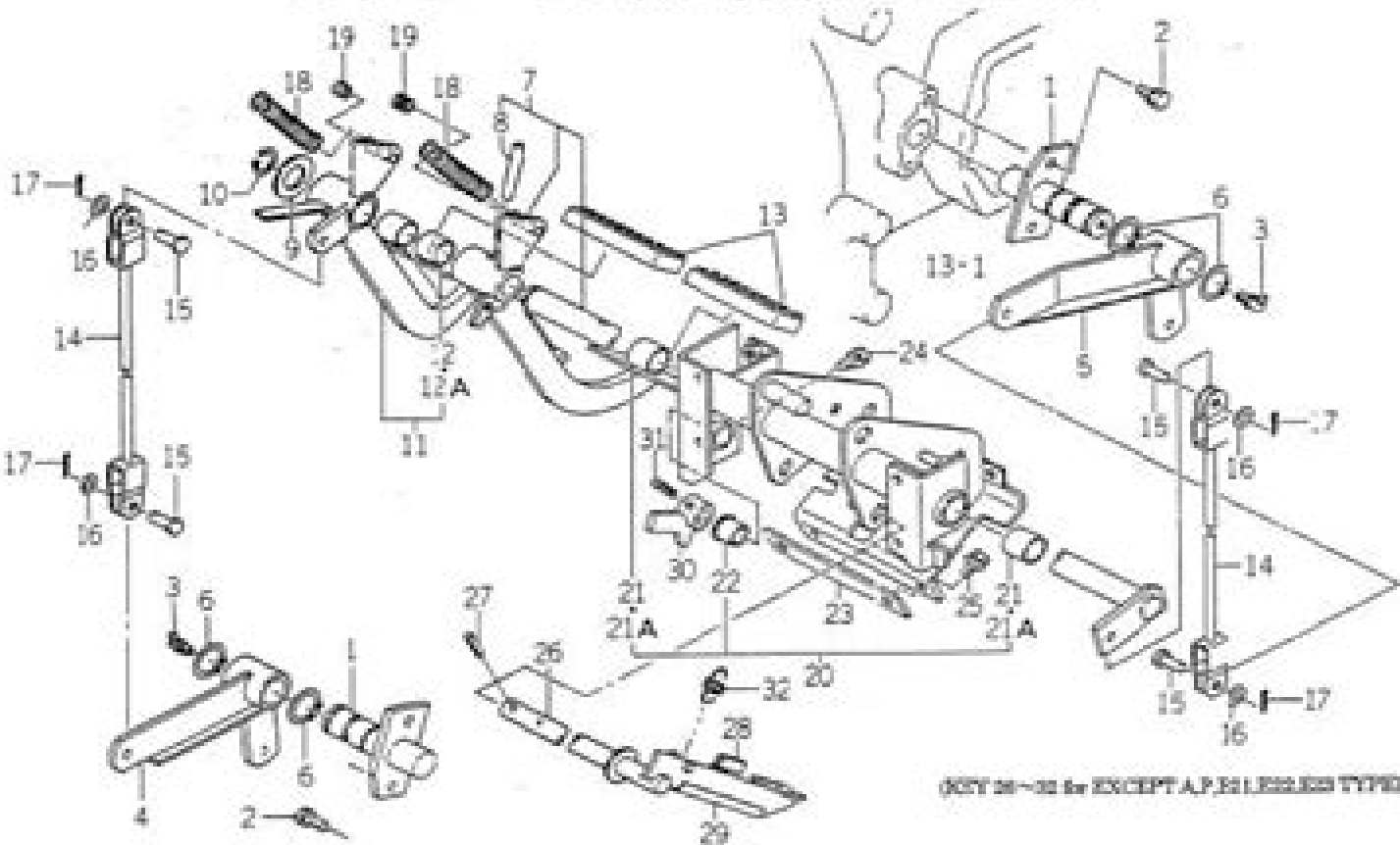
FIG. 35 BRAKE PEDAL SYSTEM
