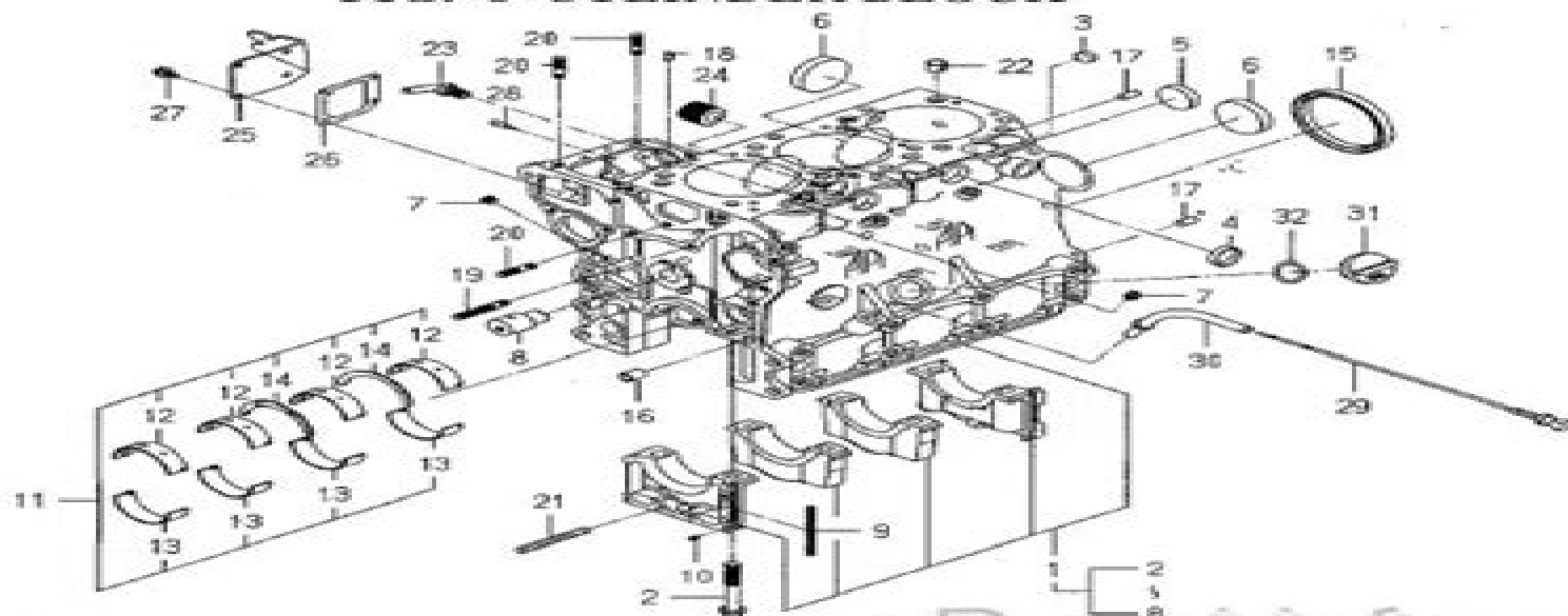
FIG. 6 CYLINDER BLOCK
