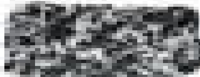
Photomicrograph of a mafic igneous rock.
