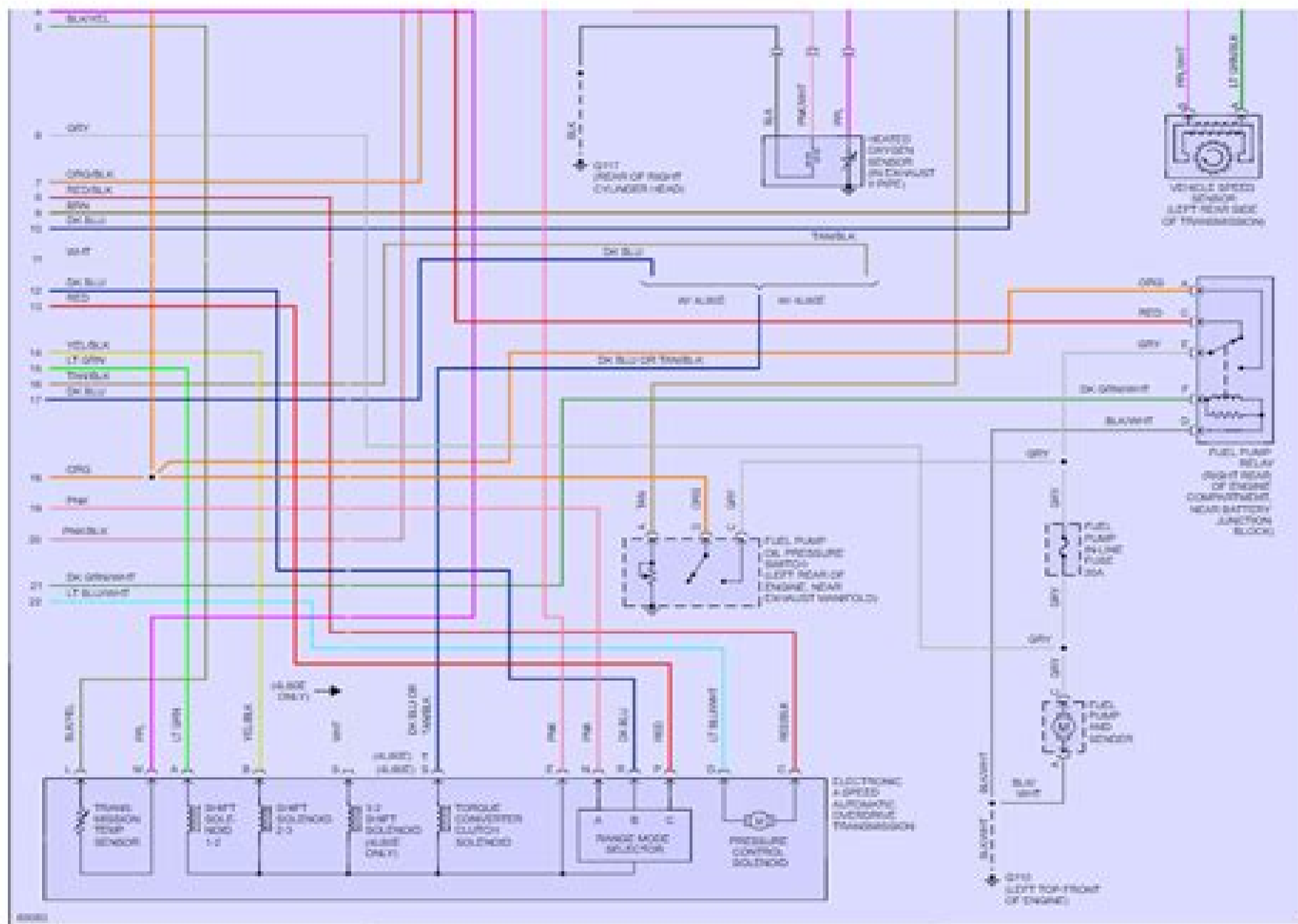
Fig 3: 5.7L (VIN K). Engine Performance Circuits, A/T (3 of 3)
