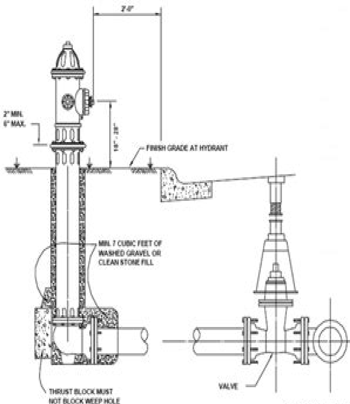
City of McKinney Standard Fire Hydrant Construction Detail
