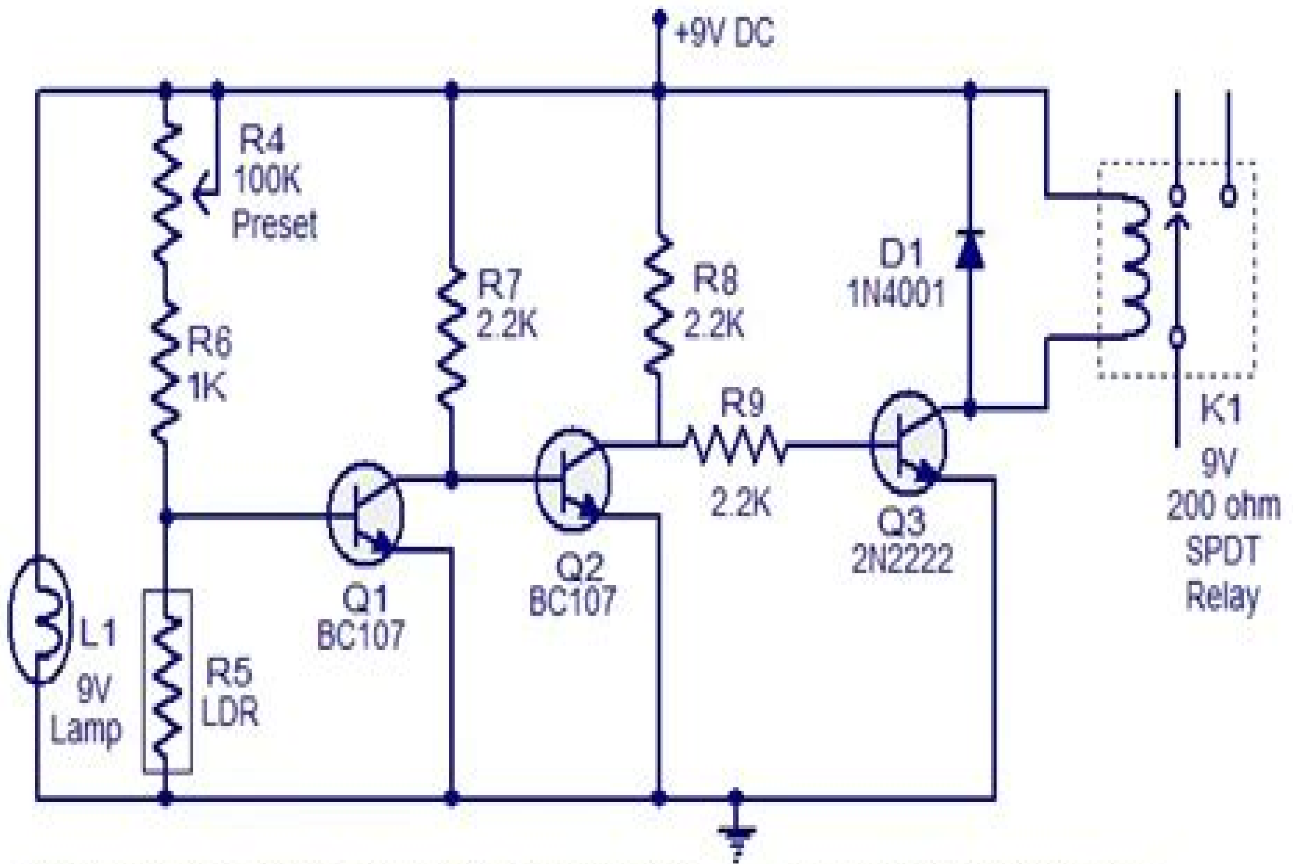
Relay version of the circuit (3 transistors)
