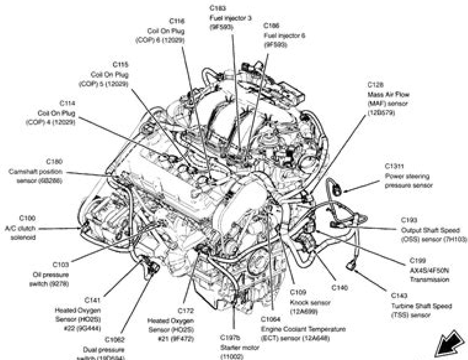
4V engine, front
