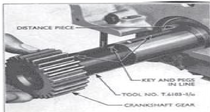
Fig. 15 Fitting the Crankshaft Gear to the Alignment Adaptor
