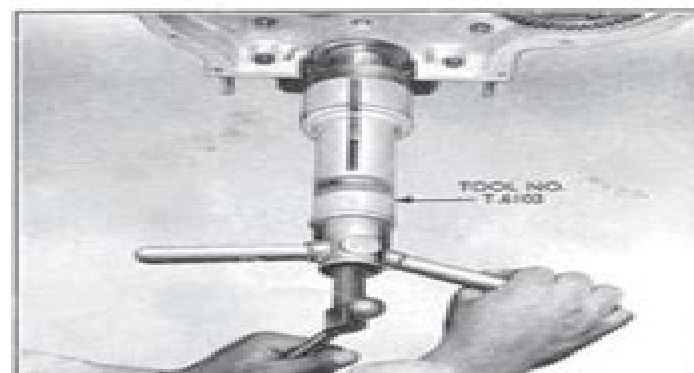
Fig. 16 Replacing the Crankshaft Gear
