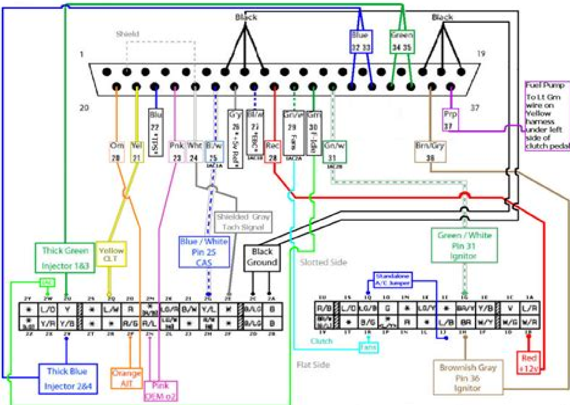
90-93 Standalone MS Harness Diagram
