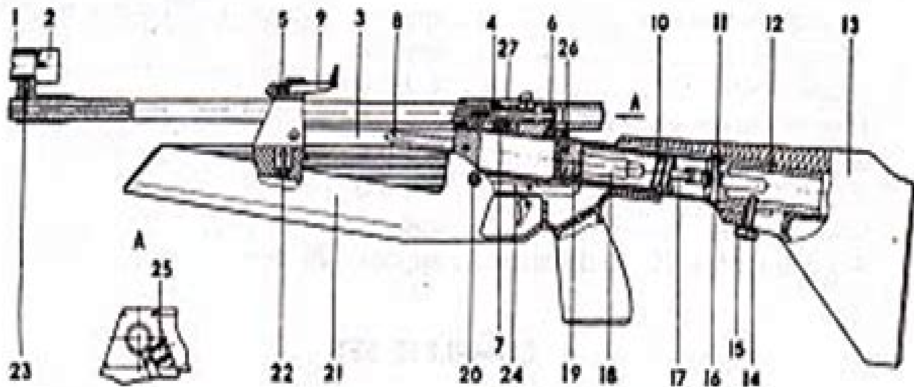
Fig.1. Scheme of the IZH-61 mechanisms
