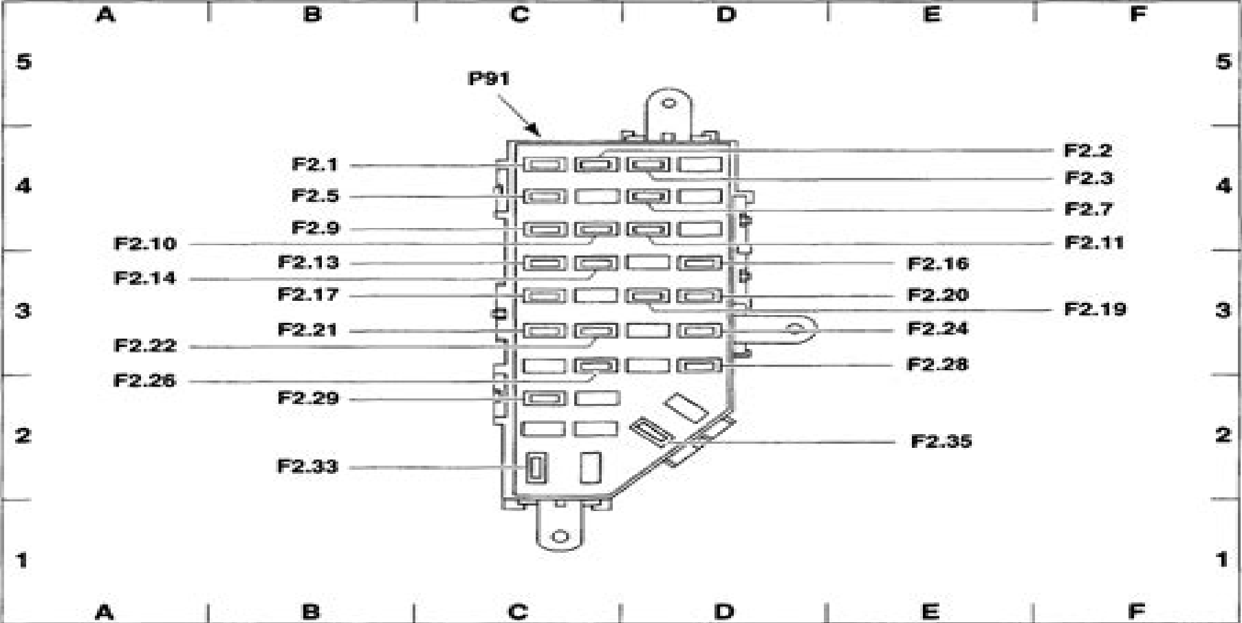
Central Junction Box (CJB)
