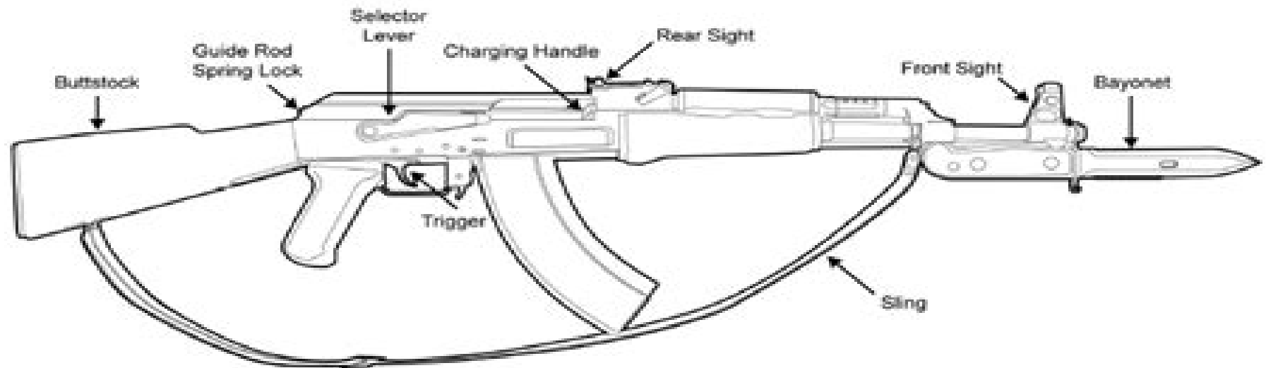
Figure 2. Right Side of the AK-47 Rifle.
