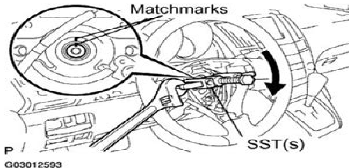
Fig. 13: Removing Steering Wheel Assy
