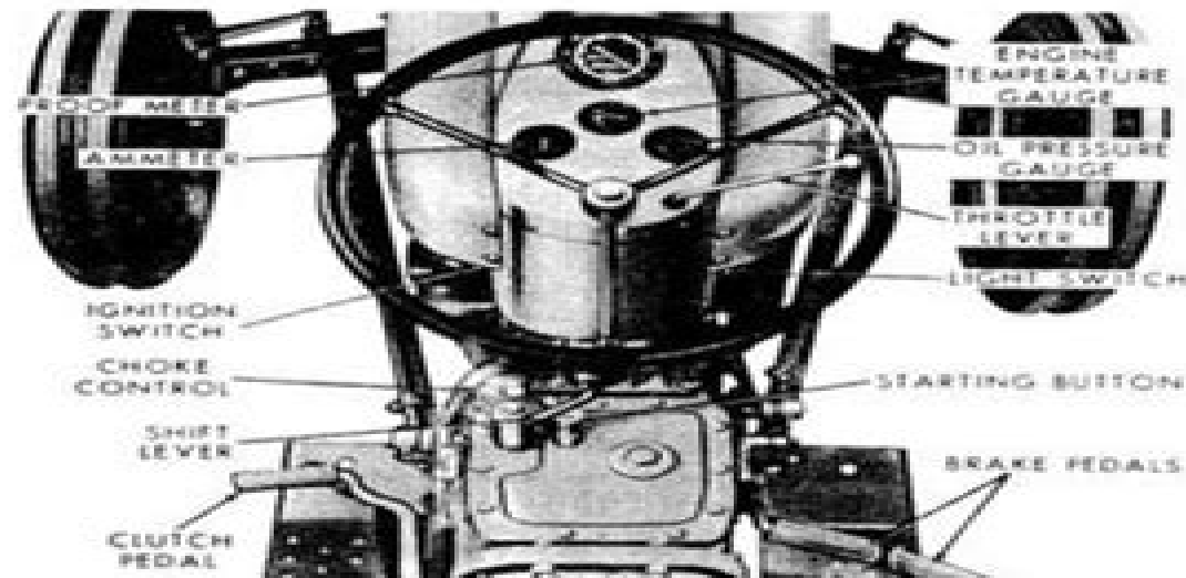
Figure 1 Controls and Instruments
