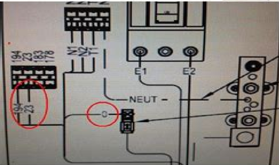
Generator Panel
