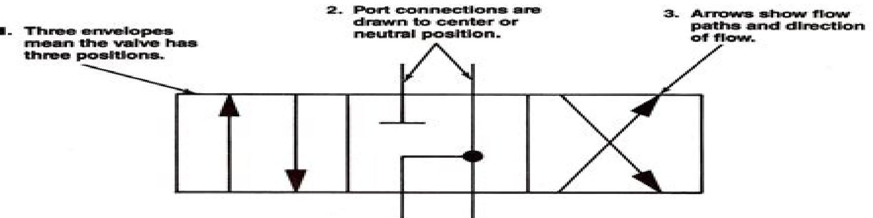
B. DIRECTIONAL VALVE (FINITE POSITIONING)
