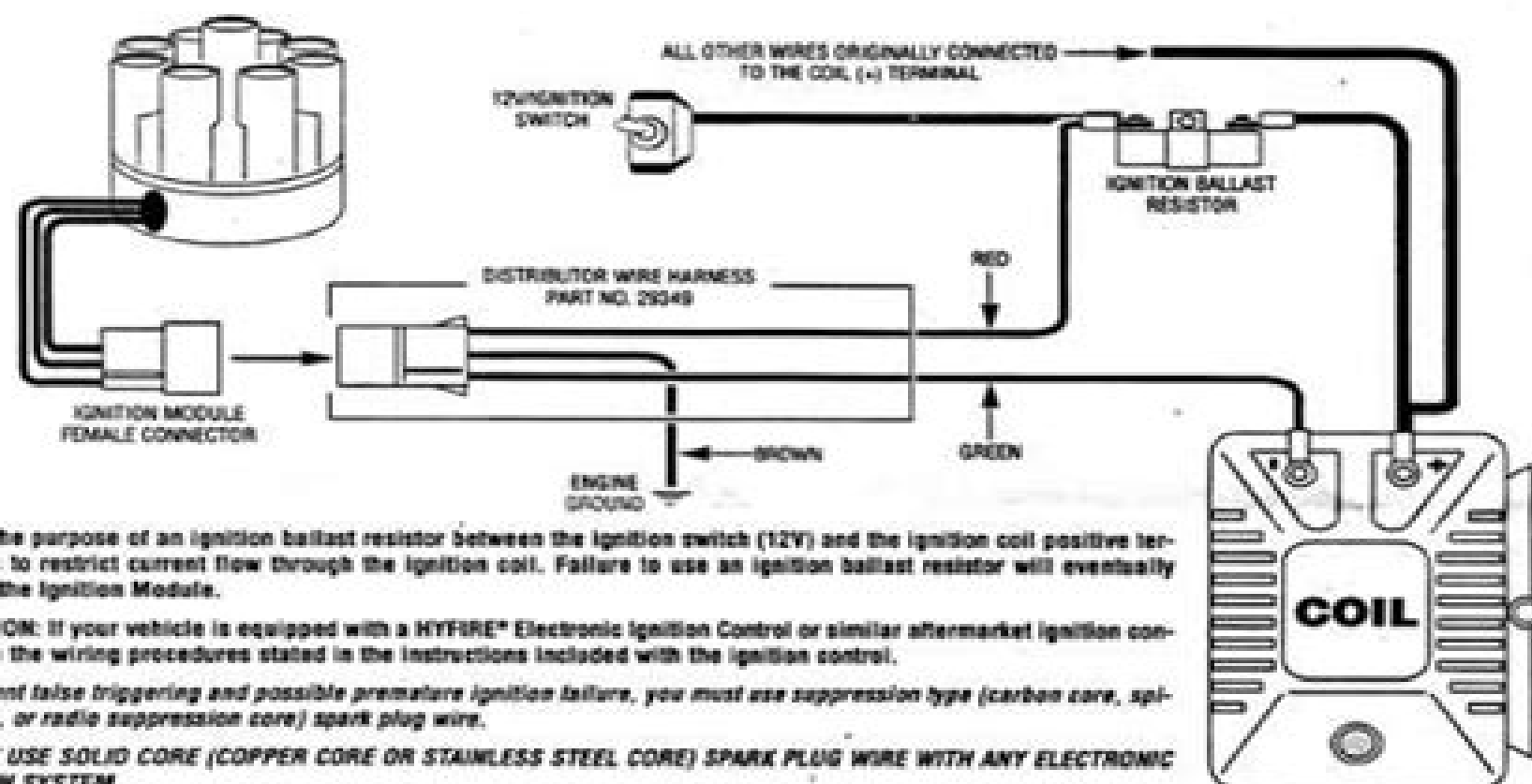
FIGURE 1 UNILITE® WIRING DIAGRAM USING BALLAST RESISTOR
