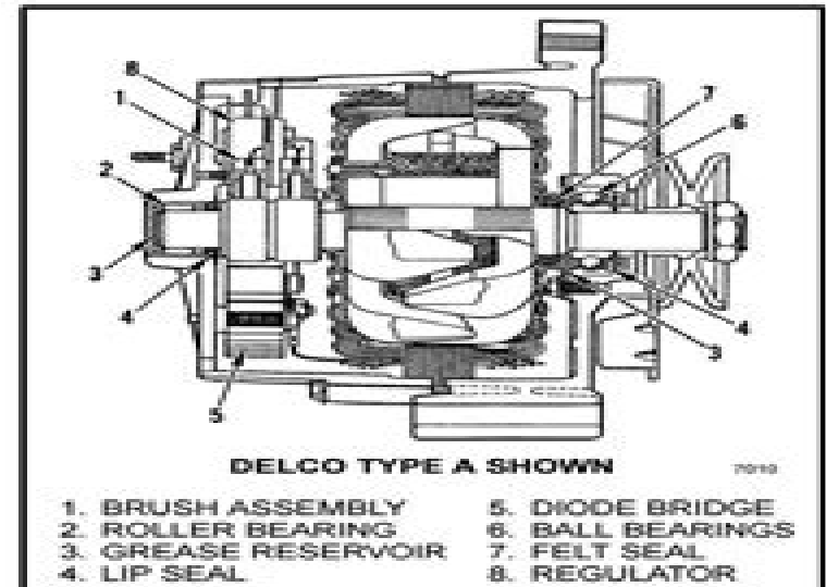
FIGURE 1. ALTERNATOR CROSS SECTION
