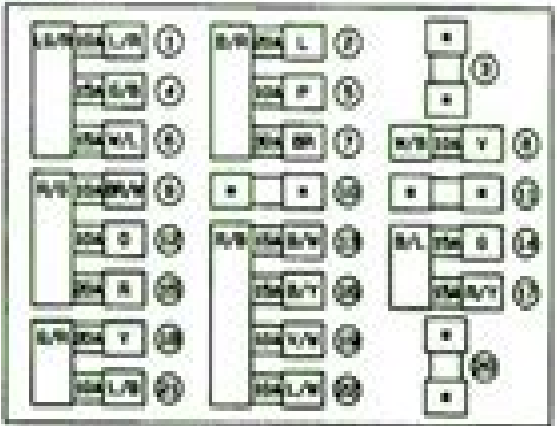
1-54 FUSE BLOCK (P)
