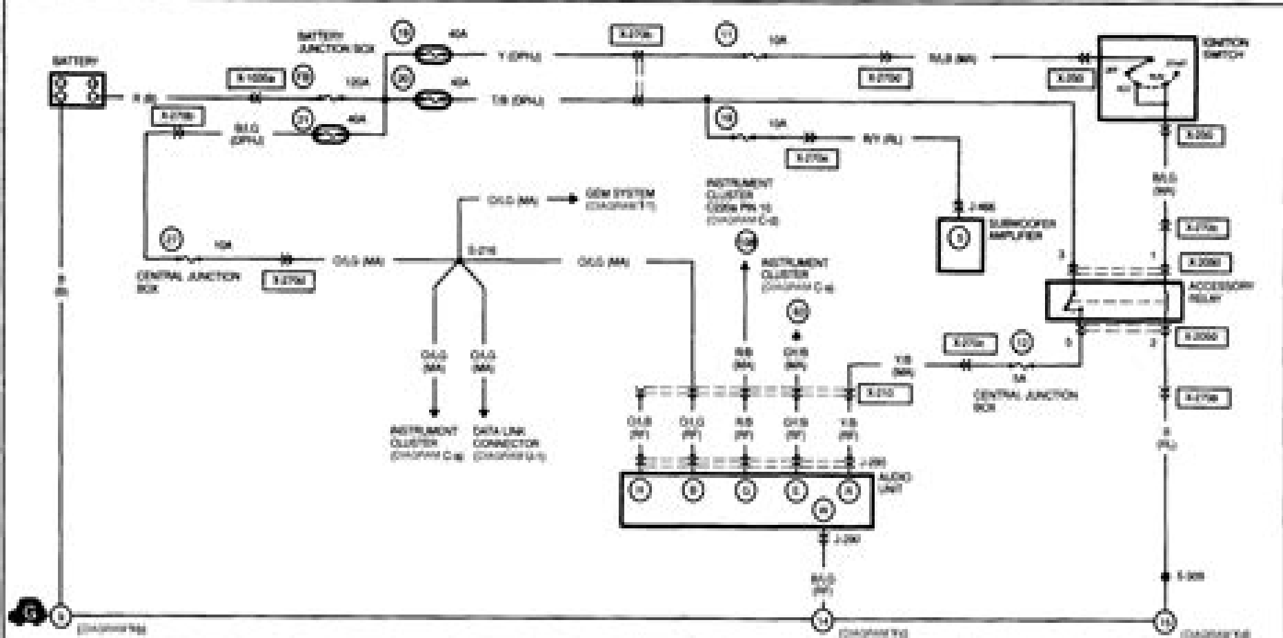
1-200 AUDIO UNIT
