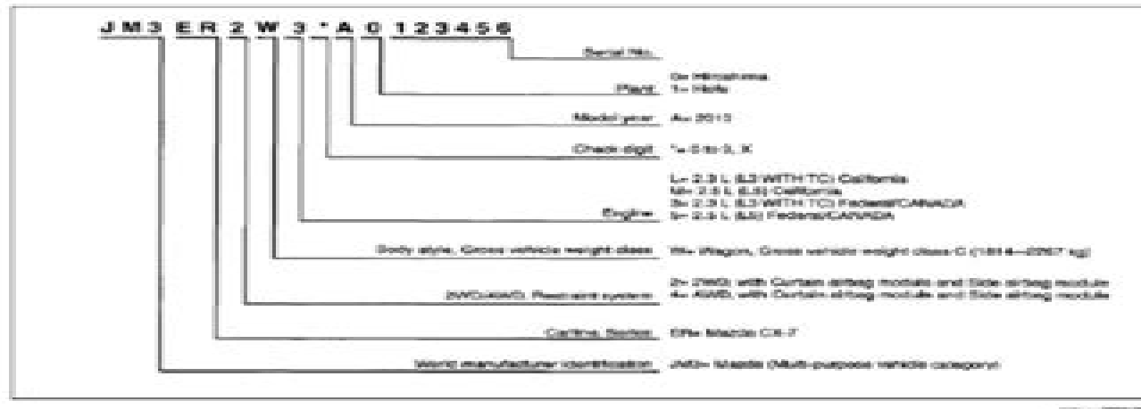
Fig. 1: Identifying Vehicle Identification Number (VIN) Code Courtesy of MAZDA MOTORS CORP.
