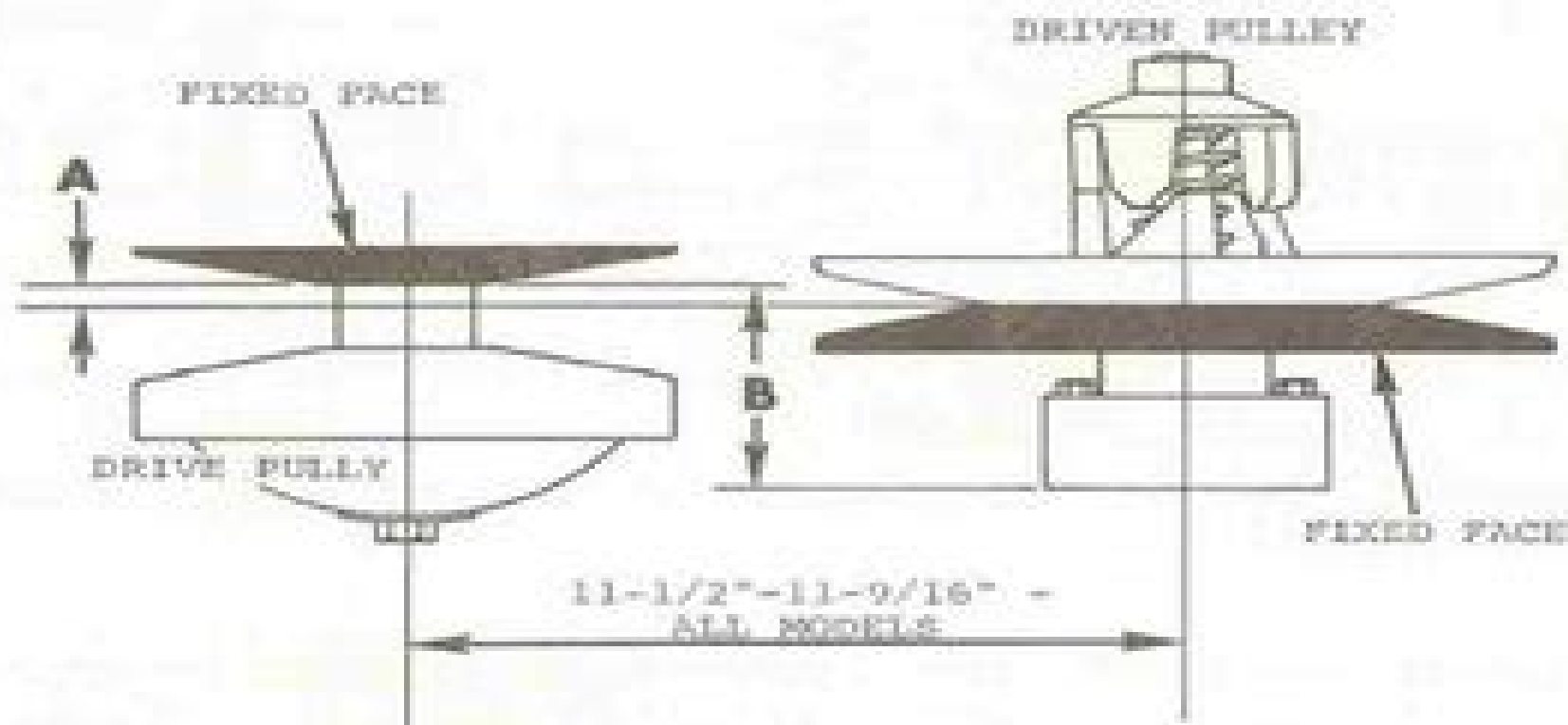
Fig. 6 — Pulley Alignment Measurements
