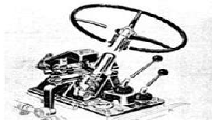
Fig. 1 — 35 Manual Steering Gear Assembly
