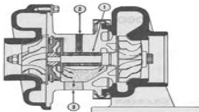
Figure 2 Turbocharger Lubrication
