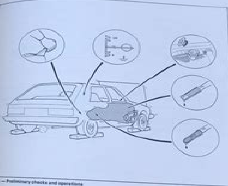
FIG. 45 — Preliminary checks and operations
