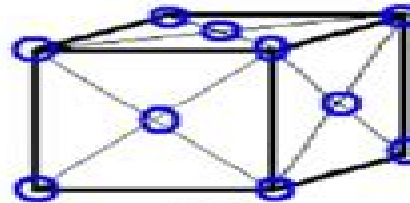
FCC
