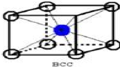
BCC
