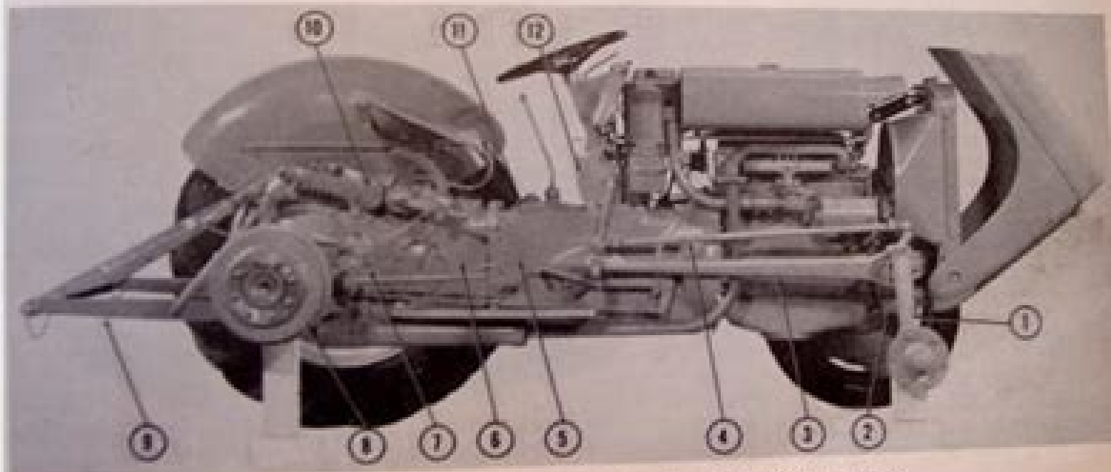
Fig. F3—Model TO35 tractor, right side view. TE35, and TO30 are similar.
