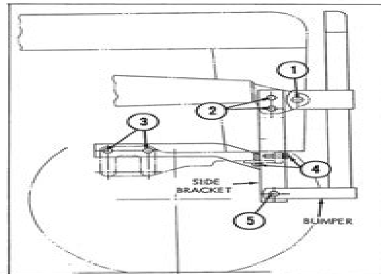
Fig. 9 - Mounting Kit Installation - MF 50 (F 40 & MH 50) and MF 65 Tractors 1. Clevis Pin (3/8" x 1 1/2") 2. Bolt (3/4" x 2-1/2" UNF) Lockwasher & Nut 3. Side Bracket 4. Bolt (3/8" x 1-1/2" UNF) Lockwasher 5. Bolt (3/4" x 2-1/2" UNF) Lockwasher & Nut
