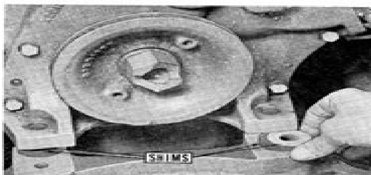
Fig. MH520—When installing the engine on models 33, 44 Special, 55 and 555, vary the number of shims until clutch shaft and transmission input shaft are aligned.
