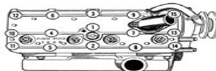
Fig. MH521 — Cylinder head nut tightening sequence for models 21 (Colt) and 23 (Mustang).
