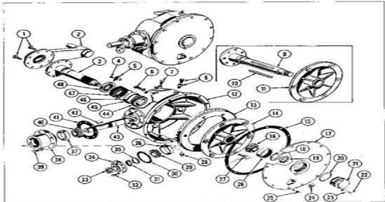
Fig. 1 — Bevel Gear Main Drive Assembly
