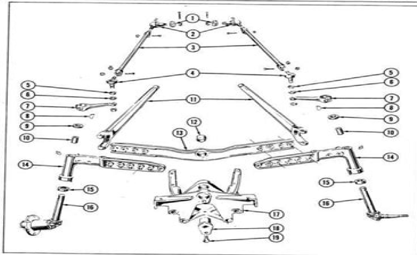
Fig. 1 - MF and TO 35 Front Axle Assembly Nomenclature
