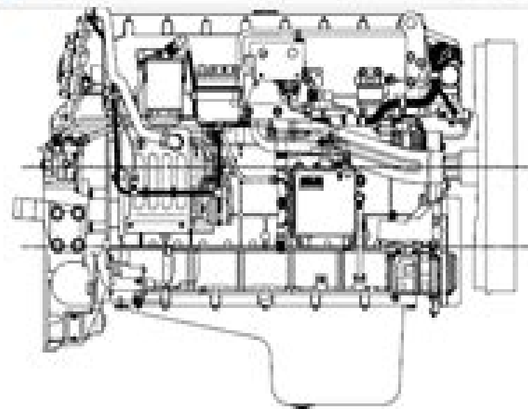
RIGHT-HAND SIDE VIEW OF THE ENGINE
