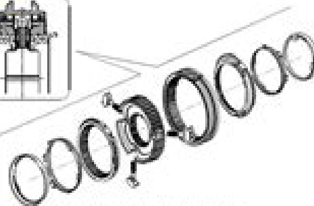
1ST AND 2ND GEAR DUAL CONE SYNCHRONIZER ASSEMBLY
