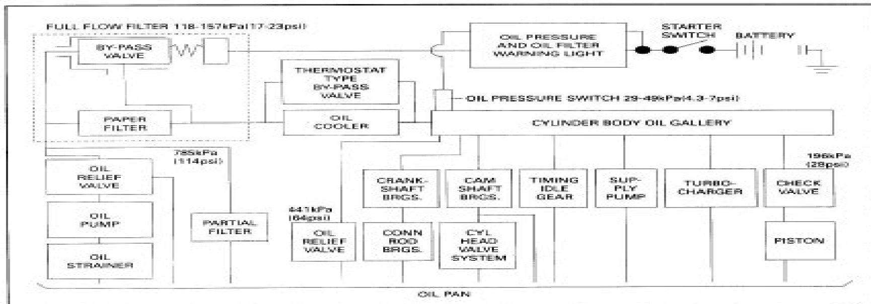
Figure 2 — Lubrication System
