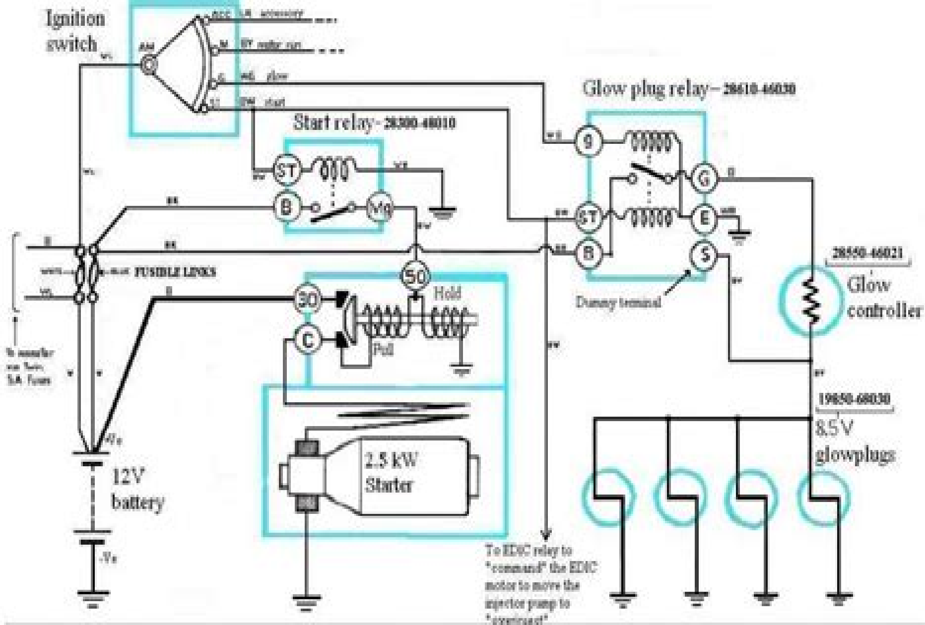
Glow/start wiring for my 1979 12 Volt Australian-market BJ40
