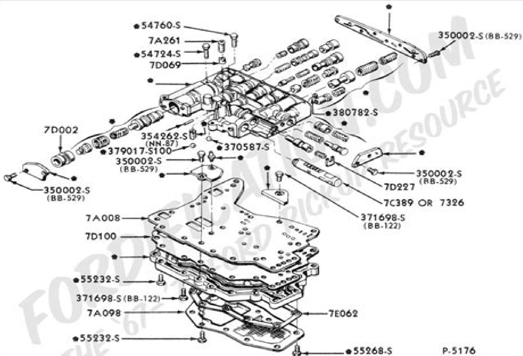
1968/72 MAIN CONTROL (C6 TRANSMISSION) - TYPICAL
