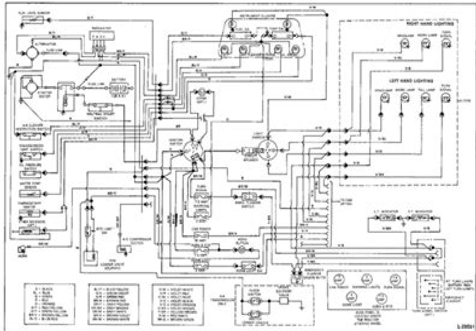
Figure 1 General Wiring Schematic
