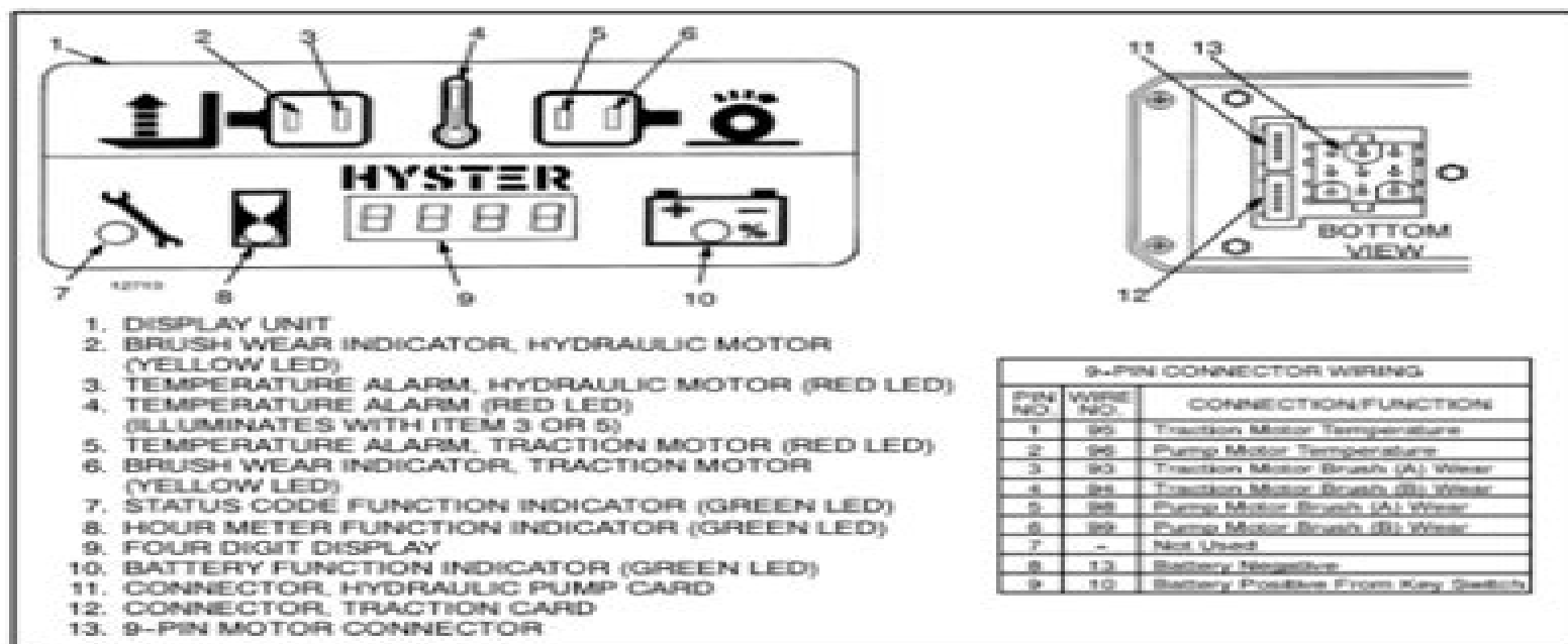
FIGURE 8. I.T.W. INSTRUMENT PANEL DISPLAY E40-60XL
