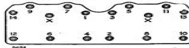
Fig. A-23— Order of tightening cylinder head bolts. Those marked X also secure the rocker shaft.
