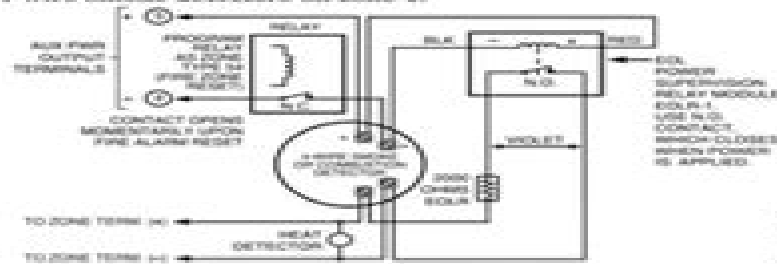
Figure 9a. 4-Wire Smoke Detector Using Relay for Power Reset
