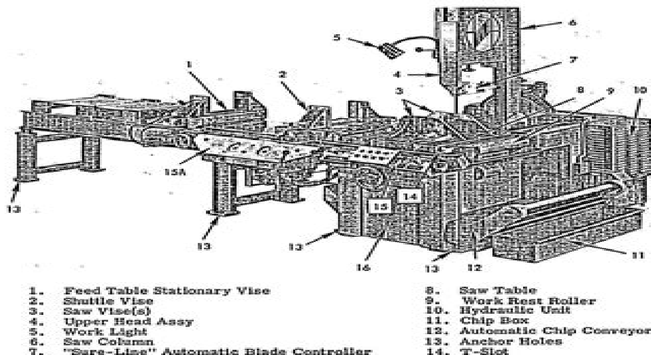
Figure 1. Series 81A Vertical Band Saw (Front View)
