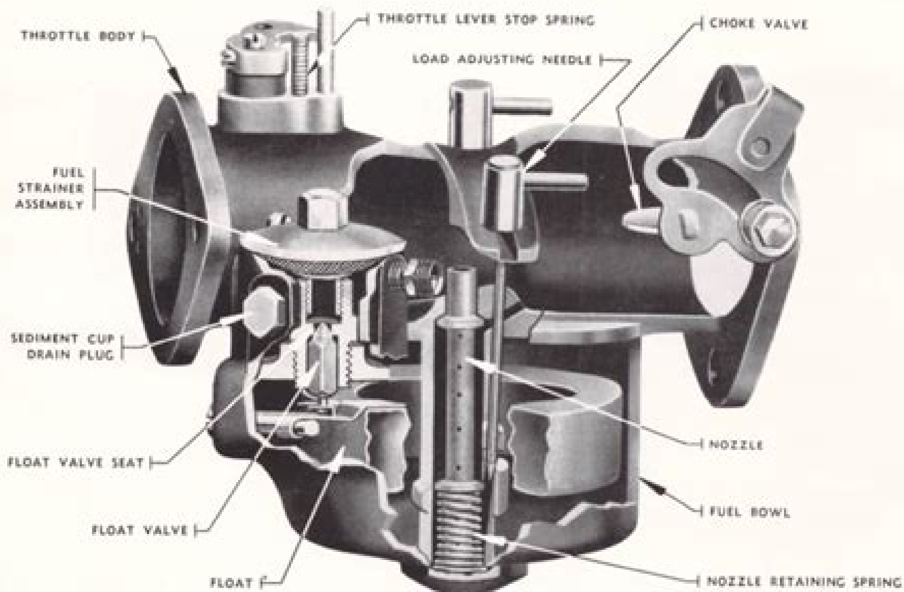
Fig. 1—Choke, Float and Power Fuel Feed Systems
