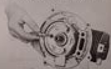
Figure 15 Shoulder Screws & Spring Installation
