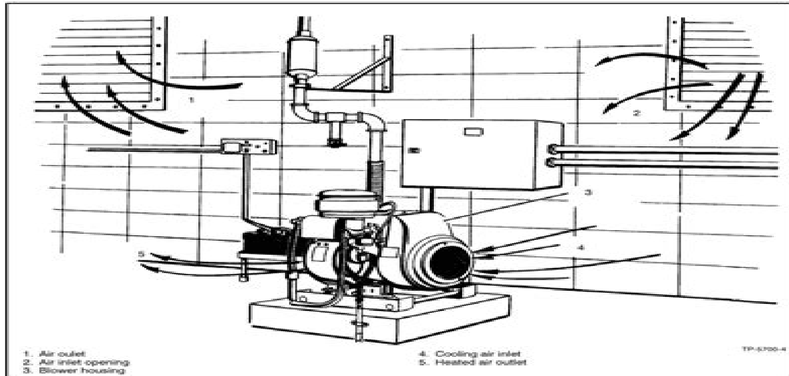
Figure 4-5 Standard Forced-Air Cooling System
