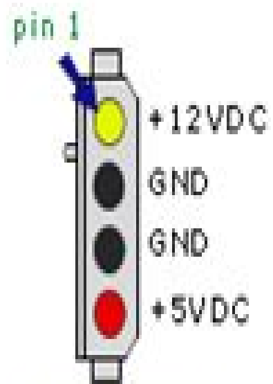
4 pin Molex peripheral Connector
