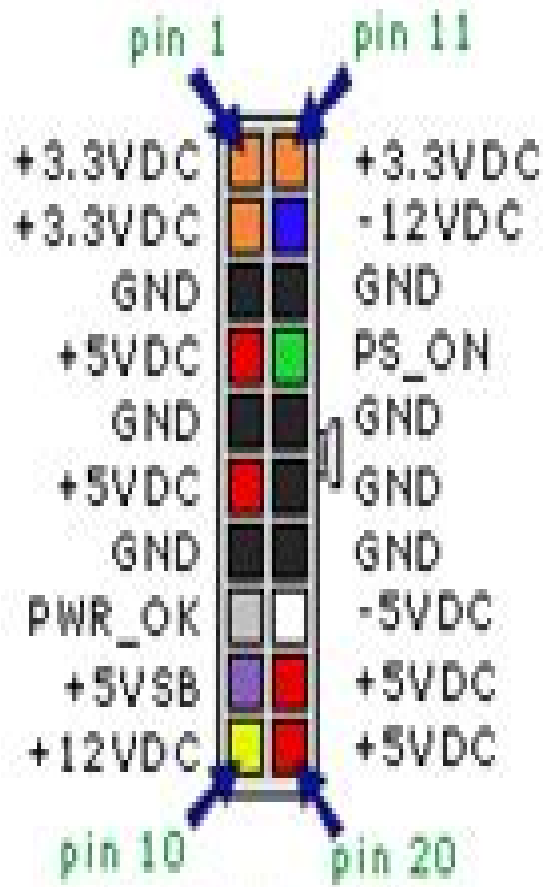
ATX 20 pin Molex Main Power Connector
