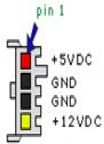
4 pin Berg Floppy Drive Connector
