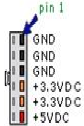
6 pin AUX Connector
