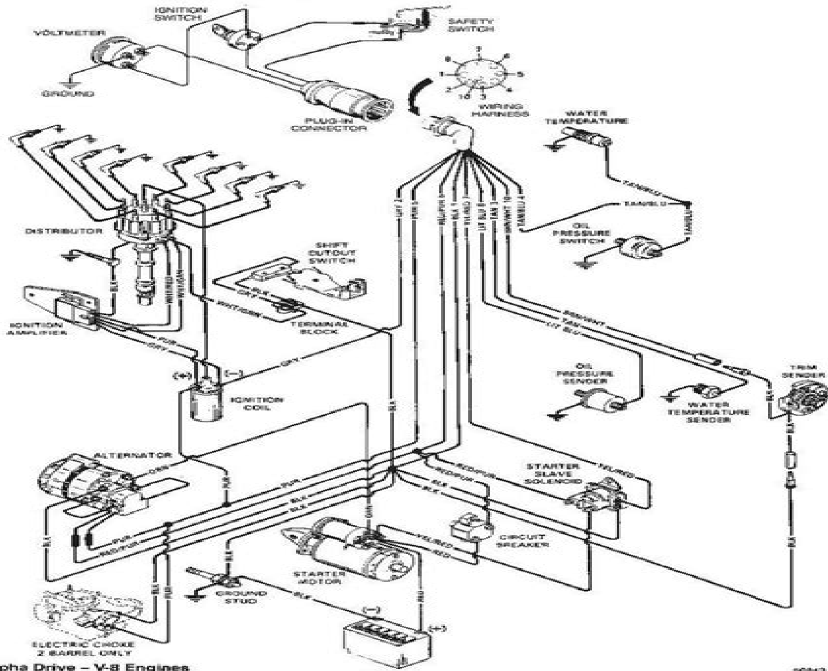
Typical Alpha Drive - V-8 Engines
