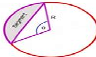
Area of a Segment = R^2/2 (\theta - \sin \theta)
