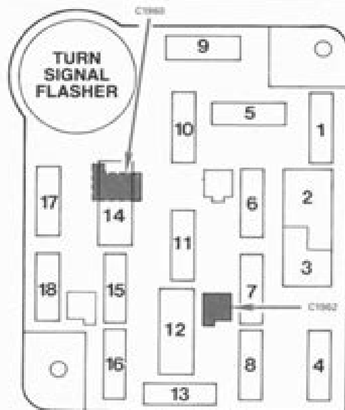
Figure 1 - Fuse Panel
