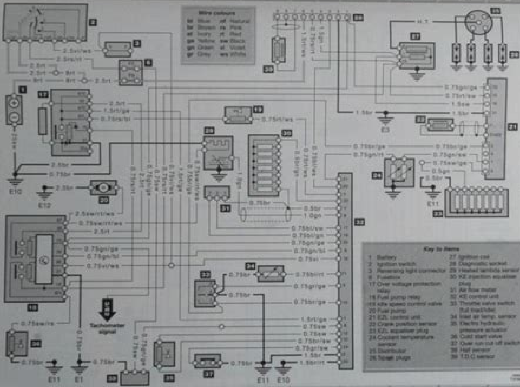
Diagram 2: Typical engine management system
