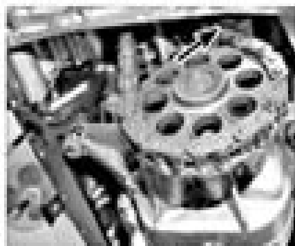
12 Place against the chain tensioner
